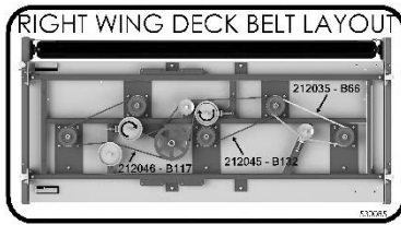
530085 RH WING DECK BELT LAYOUT
