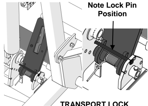
TRANSPORT LOCK POSITION - WINGS
