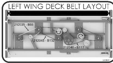
530087 LH WING DECK BELT LAYOUT
