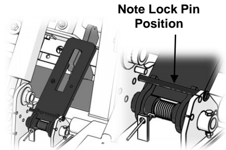
WASH-DOWN POSITION
